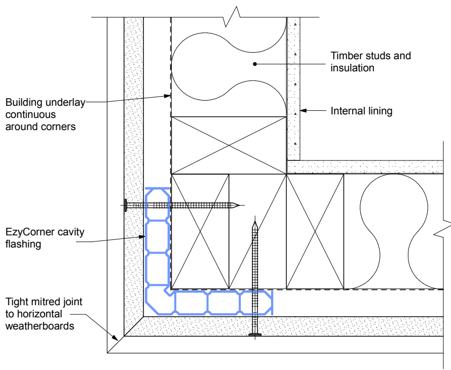
EXTERNAL CORNER
